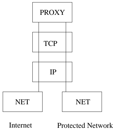
Figure 2: Overview of a application-level firewall. Data from one network pass through the proxy which forwards them to the other network if the desired security guarantees are not violated.
